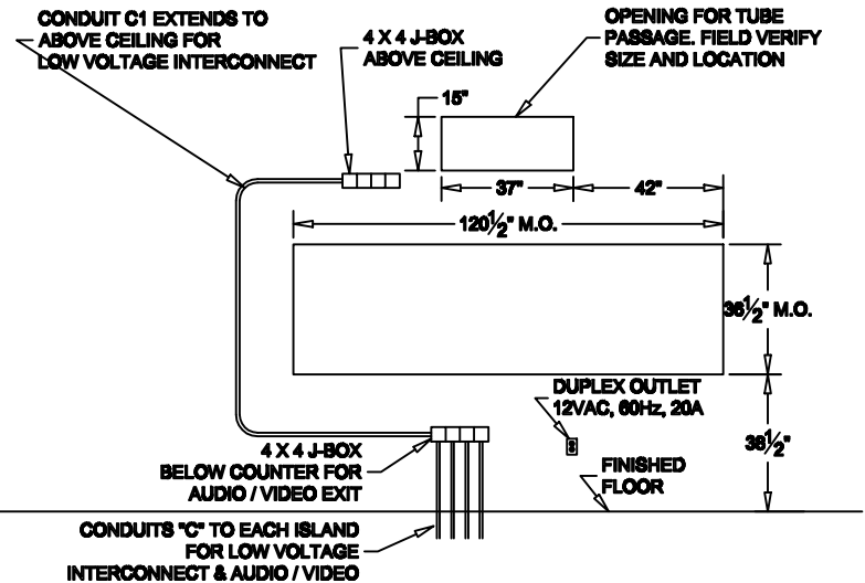
MASONRY DETAIL (FOR MODEL 310V U.L. WINDOW)
